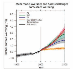
Global Surface Warming Projections, IPCC 2007
