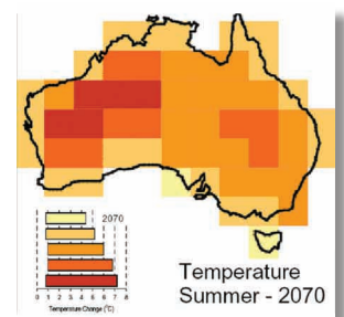
Summer Temperature Projections for Australia, CSIRO 2005
