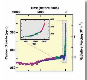
Carbon Dioxide Increase (Source: IPCC, 2007)
